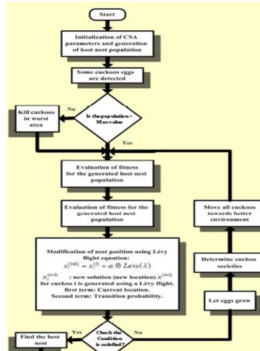
Figure 3: flow chart of cuckoo search
