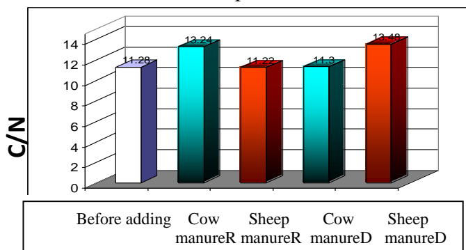
Figure 6 . Effect of organic matter on C/N values after 90 days of fermentation process
