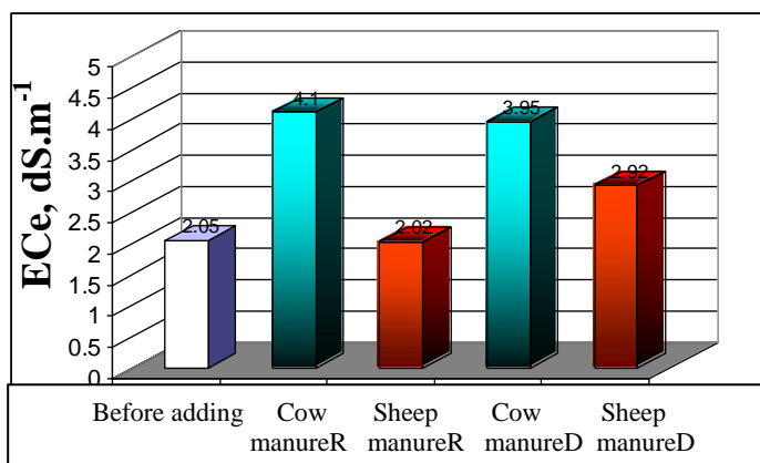
Figure 3 .Effect of organic matter on ECE values after 90 days of fermentation process
