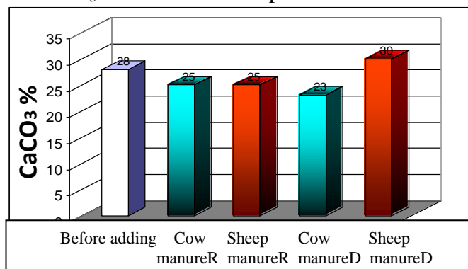
Figure 4 .Effect of organic matter on CaCO 3 values after 90 days of fermentation process
