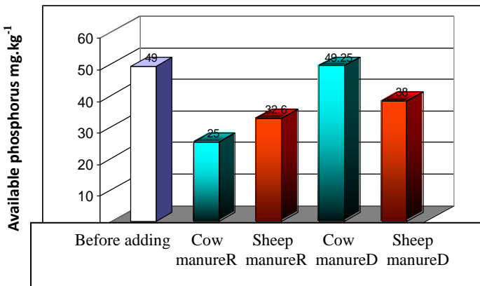
Figure 8. Effect of organic matter on available k values after 90 days of fermentation process
