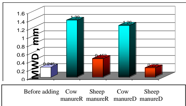
Figure 5. Effect of organic matter on MWD values after 90 days of fermentation process
