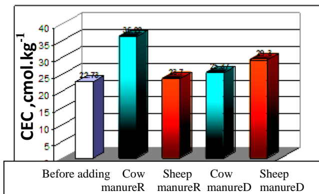
Figure 1 .Effect of organic matter on CEC values after 90 days of fermentation process
