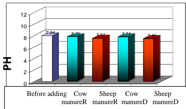
Figure 2 .Effect of organic matter on pH values after 90 days of fermentation process .
