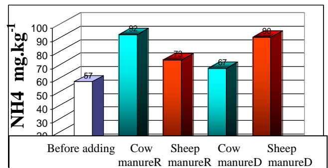
figure 7. Effect of organic matter on NH 4 values after 90 days of fermentation process
