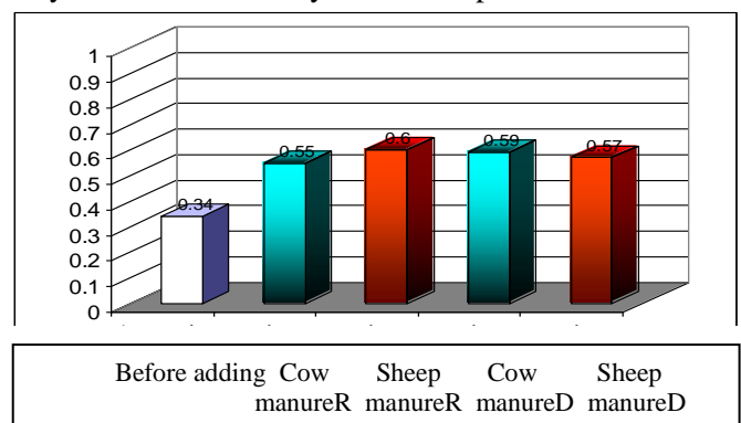
Figure 10. Effect of organic matter on hydraulic conductivity after 90 days of fermentation process
