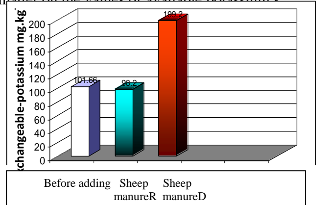
Figure 9. Effect of organic matter on soluble and exchangeable potassium after 90 days of fermentation process
